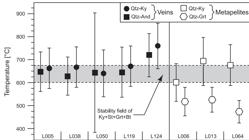
Fig. 13 Thermometry by the oxygen isotope on AbQ veins and host rocks. Uncertainties given with 2\sigma confidence. Rock samples L006 and L064 are situated in the same region as the vein samples L005, L038, L124, and L050, L119.
