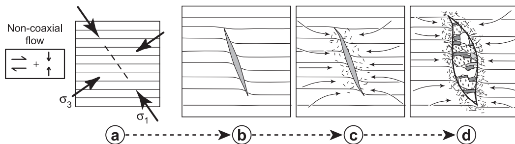
Fig. 14 Different stages of formation of the aluminosilicate tension gashes in a context of general shearing. \sigma_1 , \sigma_3 : maximal and minimal stress. When P_{\text{fluid}} is more important than the sum of tensile strength and minimal stress component, a crack can open (stages a and b). The opening yields a gradient in P, which leads to fluid migration. The fluids provoke a reaction with the host rock in the surrounding of the vein, giving rise to dissolution of alkaline and aluminous phases (stage c). The dissolved material will finally precipitate inside the vein (stage d). See text for further explanation (adapted from Etheridge, 1984; Kerrick, 1990).
