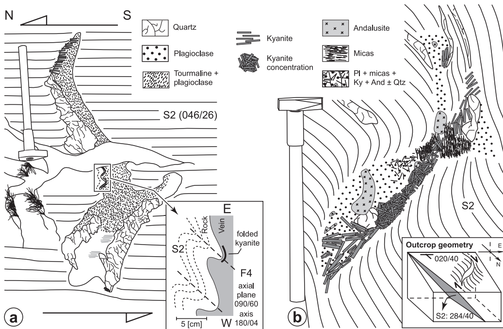
Fig. 5 Two examples of sigmoidal veins (D3 phase, Fig. 2b) with a top-to-the-north sense of shear, showing relations between D2, D3 and D4 phases (Table 1). Hammer is 60 cm long. (a) Qtz, Ky, Pl and tourmaline vein, cutting the penetrative S2 schistosity and deformed by D4 (Larecc anticline, eastern flank; Swiss coordinates: 698°710 / 137°630 / 2160 m). (b) Qtz, Pl, Ky, And and Ms vein. This outcrop is in the SW-part of the study area, on western flank of the major Larecc anticline; its orientation compared with (a) demonstrates rotation of the pre-existing veins by folding (697°925 / 137°610 / 2160 m). More examples (photos and sketches) of aluminosilicate-bearing veins are available at http://larecc.geoloweb.ch/
