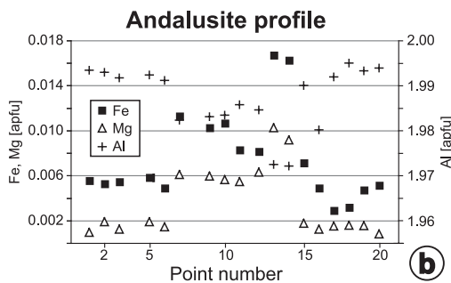
Fig. 7 (a) Distribution map of Mg for a cm-sized And crystal with Ky inclusions (sample L130). Analysis conditions: 15 kV, 20 nA, beam size = 2 μm, dwell time = 15 msec. As both Mg and Fe are correlated, this map indirectly represents also the zonation in Fe. The light-grey zone reveals the Fe-Mg-rich core of andalusite. Ky does not incorporate Mg and thus appears darker. (b) Analytical profile (total length 1.7 mm). Complete averaged analysis of rim and centre points are given in Table 2.
